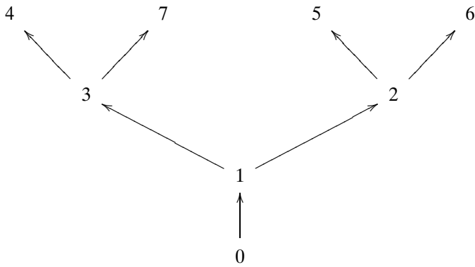
FIGURE 1. A tree.
