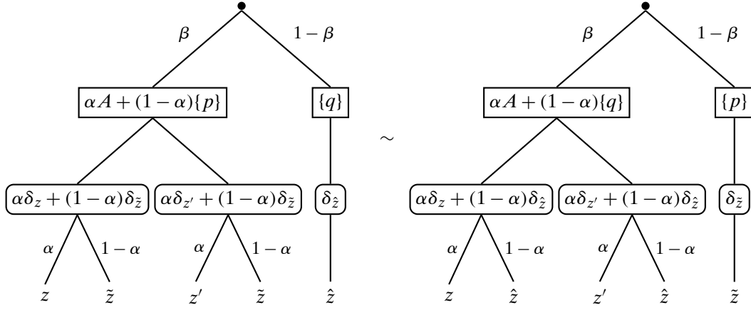
FIGURE 4. Reversibility of degenerate decisions when A = \{\delta_z, \delta_{z'}\} , p = \delta_{\bar{z}} , and q = \delta_{\bar{z}} .
