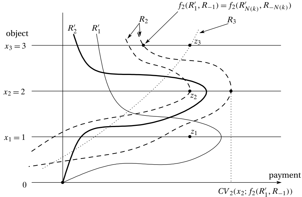
FIGURE 3. Illustration of (i), (ii), and (iii) in the proof of Proposition 2 for k = 1 .
