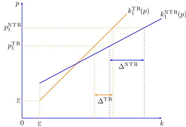
FIGURE 2. The role of the increasing hazard rate assumption.
