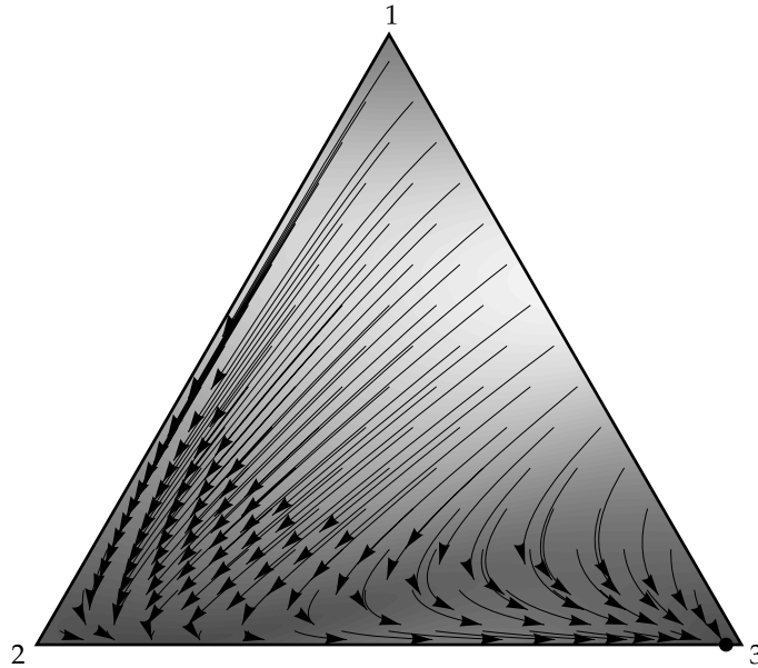
FIGURE 4. Phase diagram for the logit (0.76) dynamic in Young's game.
