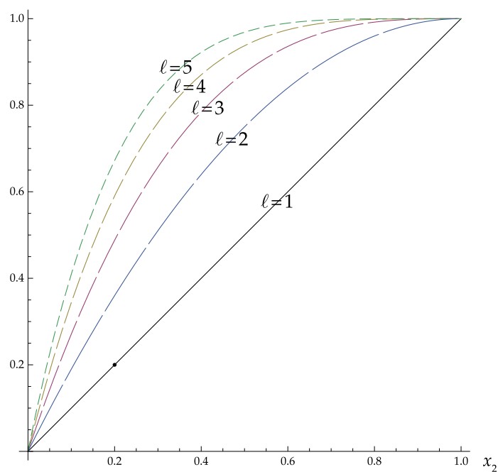
FIGURE 2. The function \mathbb{P}(\mathcal{B}_{\ell, x_2} \geq \frac{1}{5}\ell) for \ell = 1, 2, 3, 4 , and 5 .
