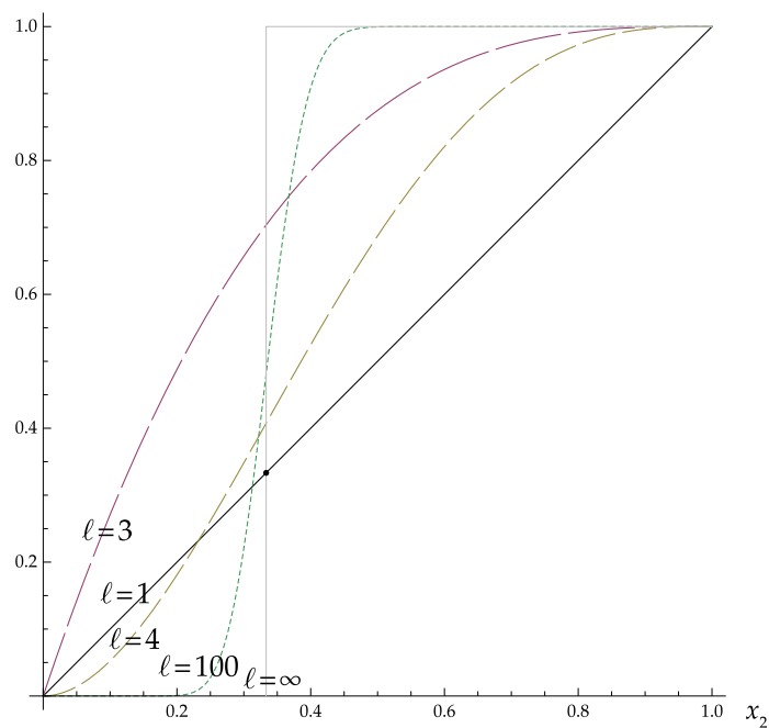
FIGURE 3. The function \mathbb{P}(\mathcal{B}_{\ell, x_2} \geq \frac{1}{3}\ell) for \ell = 1, 3, 4 , and 100 , along with the exact best response correspondence for a coordination game with mixed equilibrium x_2^* = \frac{1}{3} .
