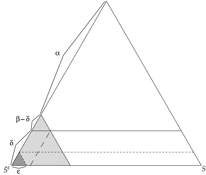
FIGURE 5. The proofs of Lemmas A.6 and A.7. The set Y^\ell is the union of the shaded regions, excluding the northwest boundary. The southern boundary of the simplex represents X_{S^{\ell-1}} . Points southeast of the dashed line satisfy x_{S^\ell} > \beta - \delta > \varepsilon .
