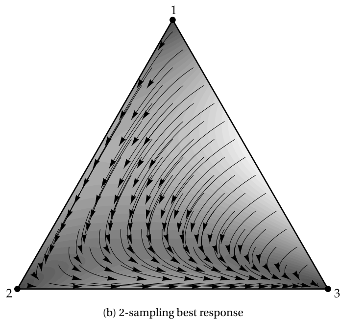
FIGURE 1. Phase diagrams for dynamics in Young's game. Grayscale represents speeds: light is fast, dark is slow.
