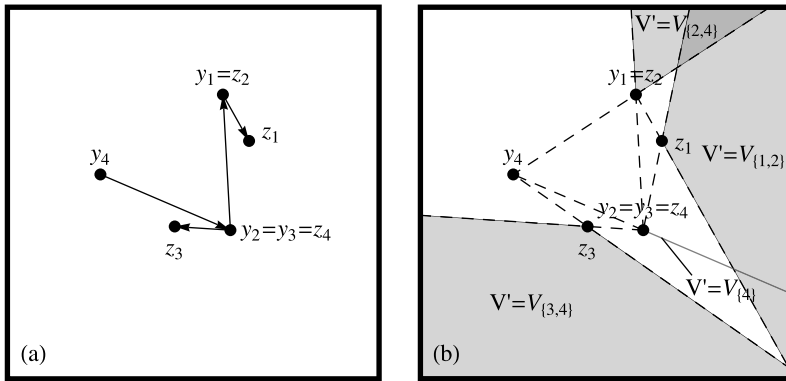
FIGURE 3. Ideal point restrictions. (a) Voting record V = \{(y_j, z_j)\}_{j=1}^4 ; an arrow emanating from y and pointing to z indicates (y, z) \in V . (b) The voter with voting record V of (a) cannot have a (strictly) (quasi)concave utility function with ideal point that lies in the gray areas. For each \hat{x} in these areas, condition (\hat{S}) is violated for the indicated restricted voting record V' .
