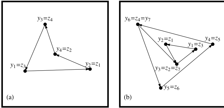
FIGURE 2. Rationalizability and admissible cycles. An arrow emanating from y and pointing to z indicates (y, z) \in V . (a) V = \{(y_j, z_j)\}_{j=1}^4 violates (W) because the indifference contour crossing y_1, \dots, y_4 cannot delineate a convex set. (b) V = \{(y_j, z_j)\}_{j=1}^6 satisfies (W) but V = \{(y_j, z_j)\}_{j=1}^7 does not since the nested indifference contour crossing through y_1, y_2, y_3 cannot be ranked above the contour crossing through y_4, y_5, y_6 .
