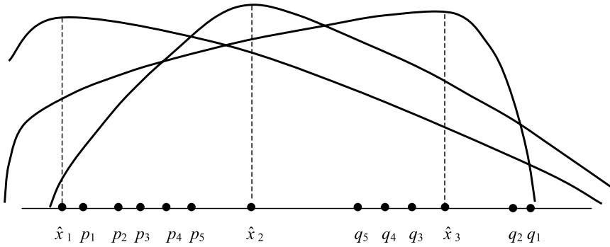
FIGURE 4. Illustration of Theorem 4. An example of the construction in the proof of Theorem 4 for n = 3 voters, m = 5 voting items, and ideal points that satisfy \hat{x}_1 < \hat{x}_2 < \hat{x}_3 . The voting alternatives are located so that condition (S 1 ) is satisfied for any voting decisions by these voters. In this example, the voting decisions are given by v_j^1 = \text{yes} for all j = 1, \dots, 5 for voter 1, v_1^1 = v_3^2 = v_4^2 = \text{no} and v_2^2 = v_5^2 = \text{yes} for voter 2, and v_3^3 = v_4^3 = v_5^3 = \text{no} and v_1^3 = v_2^3 = \text{yes} , for voter 3.
