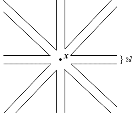
FIGURE A3. The \hat{d} -neighborhood of x when m = 2 and T = 2 in Example 1 .
