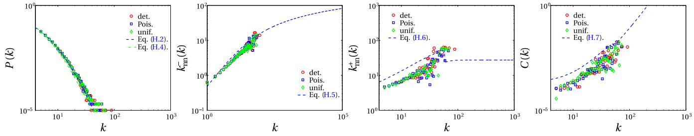
FIGURE S2. Comparison of simulation results with theoretical prediction of the link formation process in Definition S3 under global information with p = 0.5 , m = 4 , \beta = 0.1 , and T = 10^5 . Simulation results for the deterministic case ( \circ ), a uniform distribution X_m \sim U\{1, 2m - 1\} ( \diamond ), and a Poisson distribution X_m \sim \text{Pois}(m) ( \square ), both with expectation \mathbb{E}(X_m) = m are shown.
