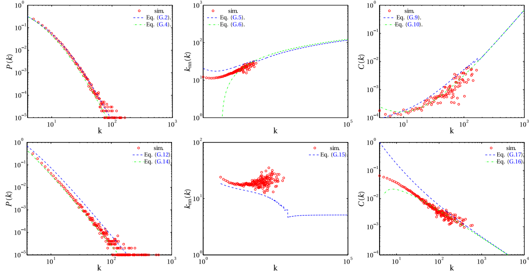
FIGURE S1. Top row: Comparison of simulation results with the theoretical predictions for T = 10^5 , S_t = \mathcal{P}_{t-1} , and m = 4 , with \beta = 0.1 under the linear approximation to the attachment kernel. Bottom row: Comparison of simulation results for T = 10^5 and n_s = m = 4 ( \beta = 0 ) with the theoretical predictions. Comparing the results of global and local information, we find that they differ mainly in the clustering degree distribution.
